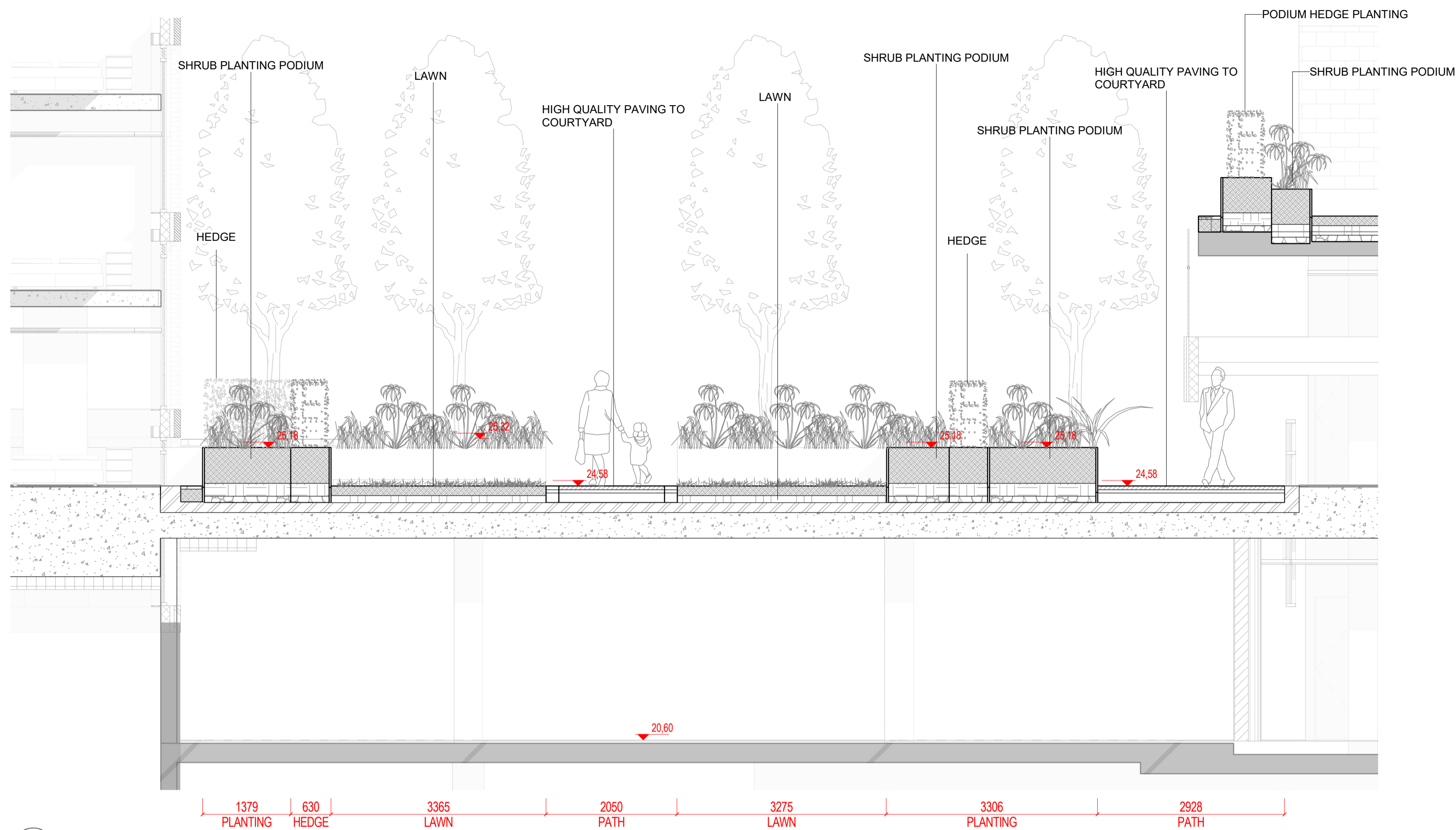
1 COURTYARD SECTION - BG2 1 1:50 @A1
