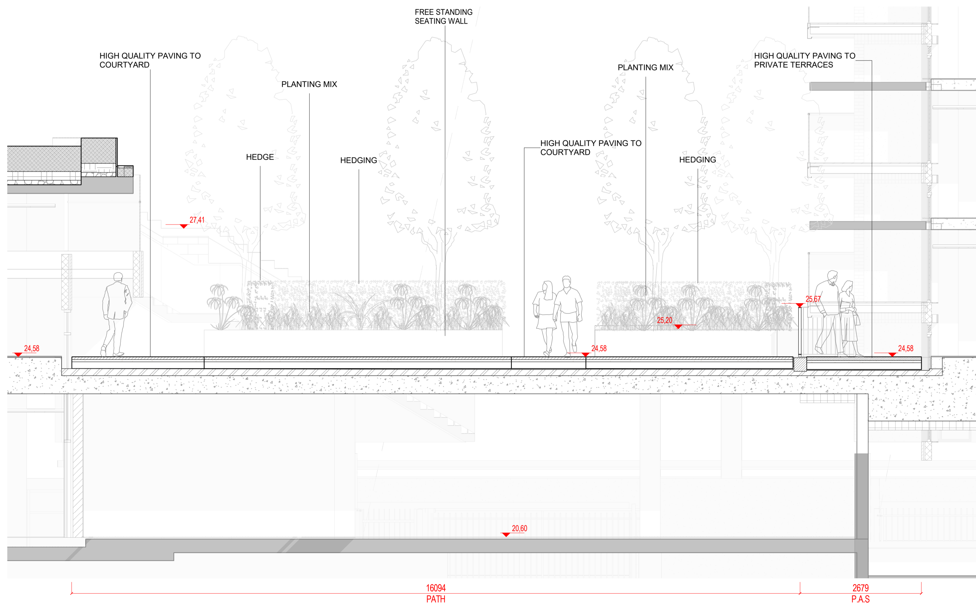
2 COURTYARD SECTION - BG2 2 1:50 @A1
